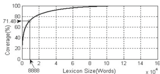
Fig. 2 Words usage frequency distribution
