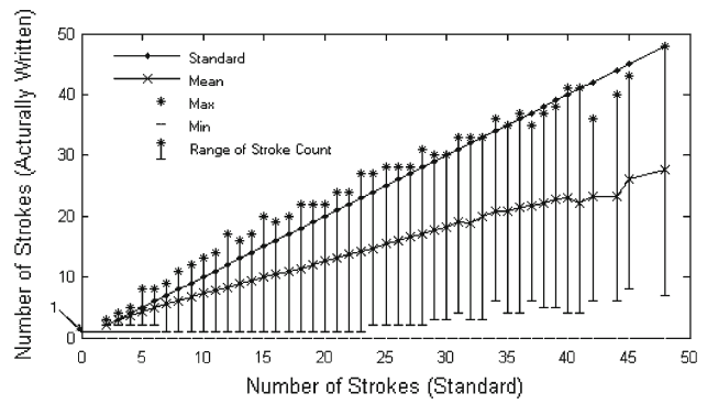
Fig. 11 Statistics on words stroke numbers
