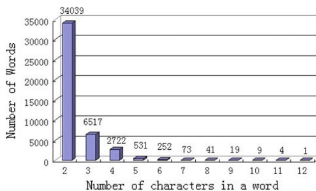
Fig. 4 Statistics of lengths of words in Word44208 dataset
